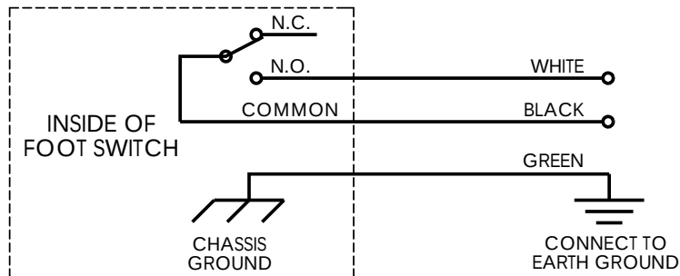
MODELS WITH LEADS (EXAMPLE: G500-MO-1502)
