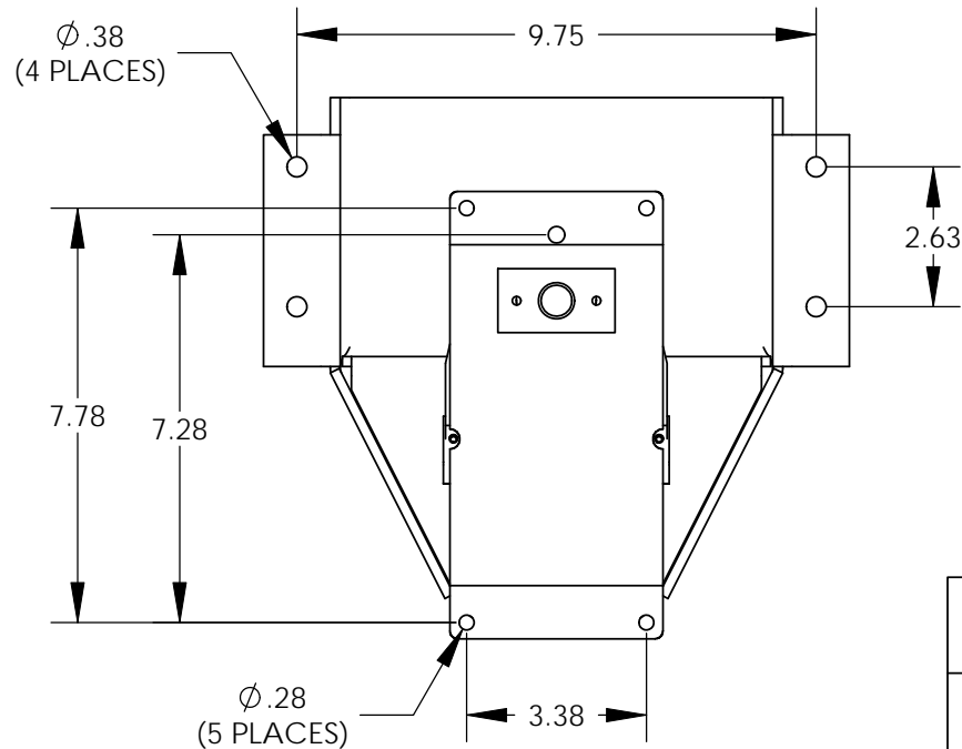
BASE MOUNTING HOLE PATTERN
