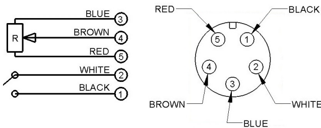
PLUG END VIEW
