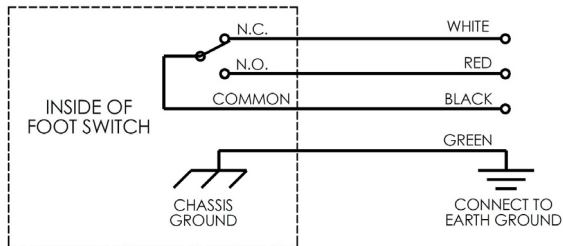
WIRING DIAGRAM: SHOWN IN THE AT-REST OR UPRIGHT POSITION.
